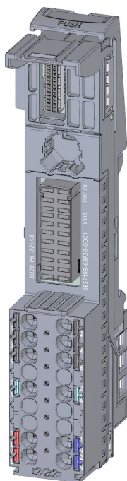
Figure 7-23 BU type C1, dark-colored version, with AUX terminals, supply over P1, P2 busbar
