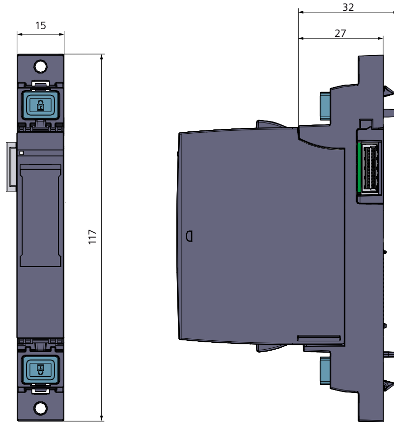
Figure B-1 Dimension drawing BC type A0, light-colored version
