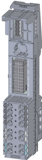
Figure 7-27 BU type F0, dark-colored version, with AUX terminals, supply over supply terminals
