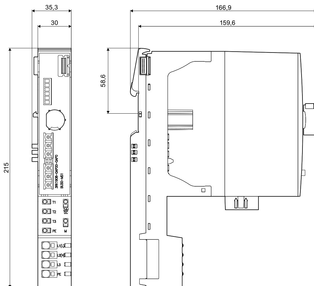
Figure D-1 Dimension drawing BU30-MS1
