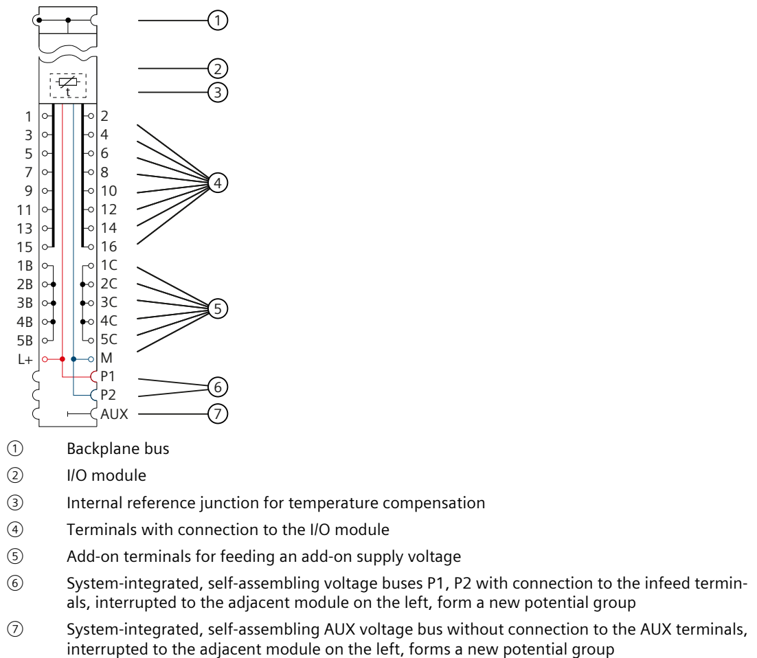
Figure 7-10 Block diagram BU type A1, light-colored version, with add-on terminals
