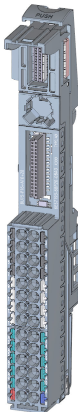
Figure 7-5 BU type A0, dark-colored version, with AUX terminals
