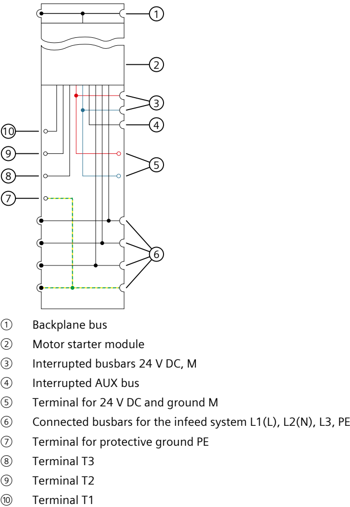
Figure 8-6 Block diagram BaseUnit with 24 V DC infeed
