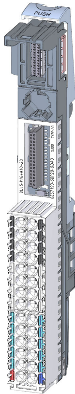
Figure 7-1 BU type A0, light-colored version, with AUX terminals
