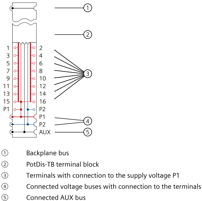
Figure 9-4 Block diagram of the PotDis-BU type P1, dark-colored version
