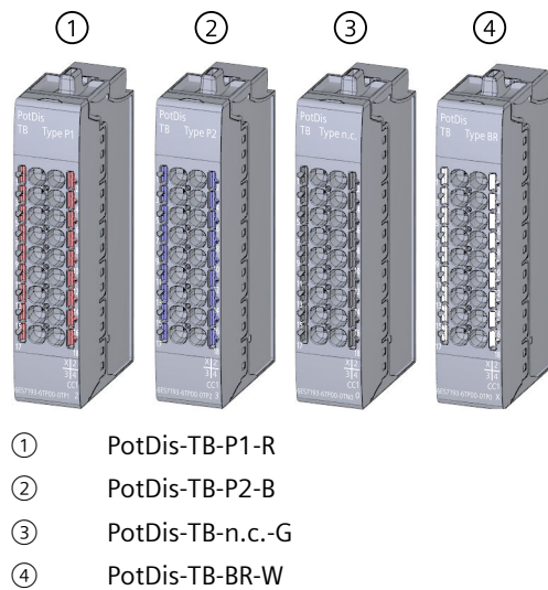
Figure 9-9 PotDis terminal blocks
