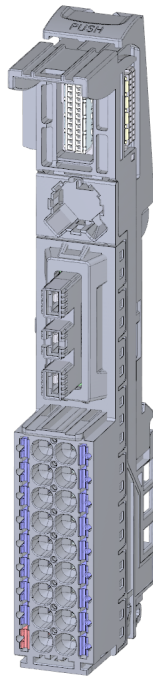
Figure 9-7 PotDis-BU type P2, dark-colored version
