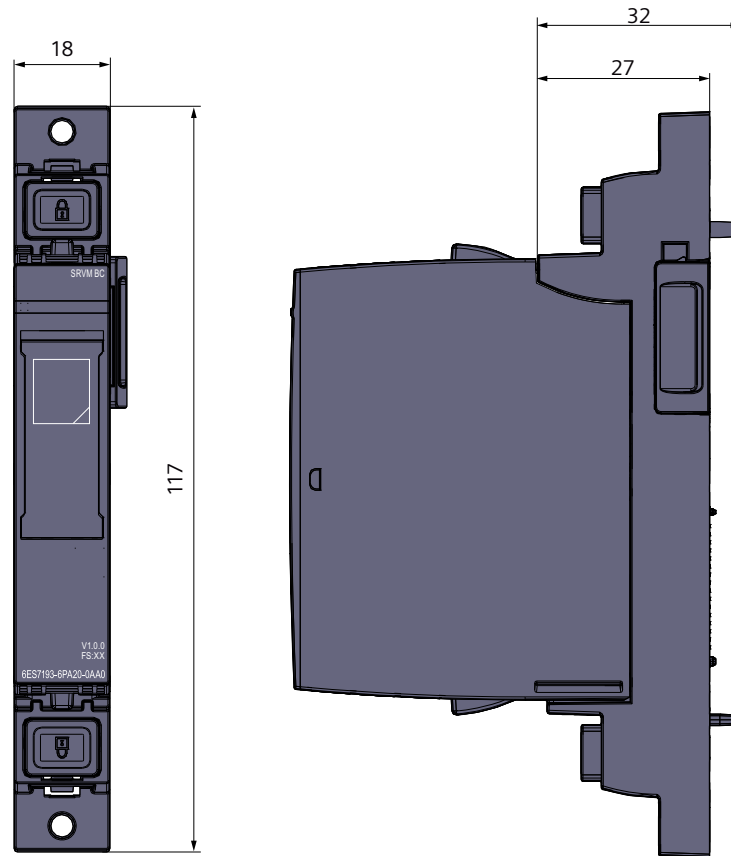
Figure B-3 Dimension drawing BC type A0, BaseCarrier for server module
