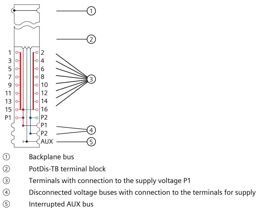
Figure 9-2 Block diagram of the PotDis-BU type P1, light-colored version
