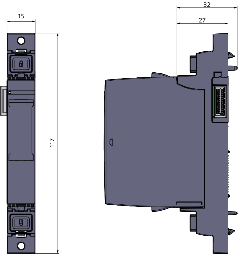
Figure B-2 Dimension drawing BC type A0, dark-colored version
