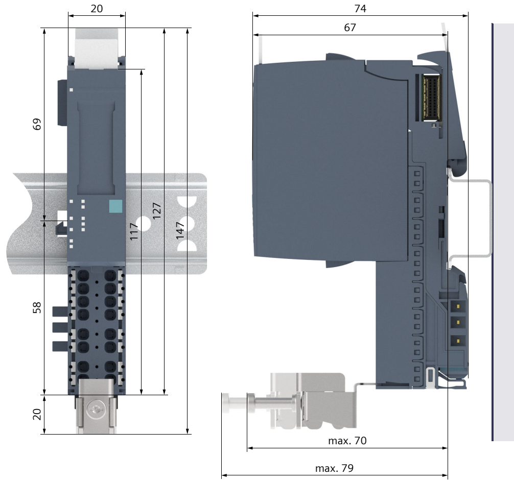
Figure C-3 Dimension drawing BU20-P12+A4+0B
