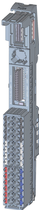
Figure 7-13 BU type A1, dark-colored version, with add-on terminals
