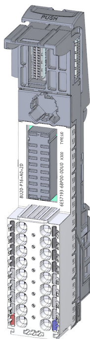
Figure 7-29 BU type U0, light-colored version without AUX terminals
