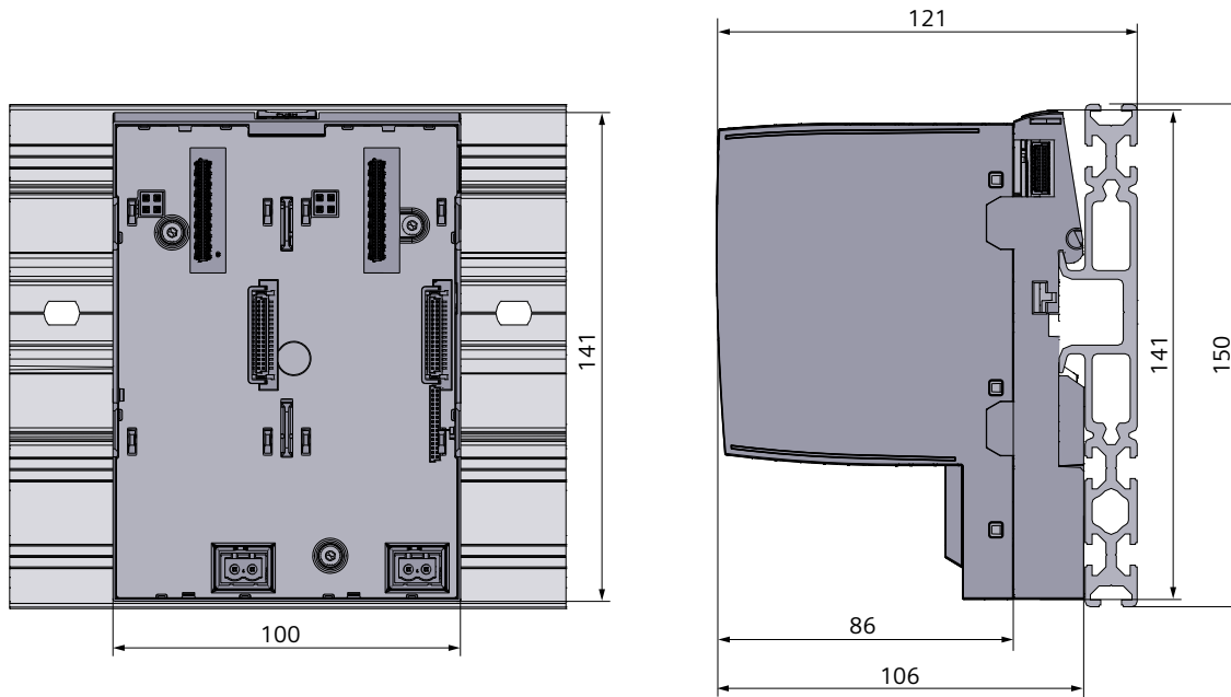
Figure A-1 Dimension drawing of BU type M0
