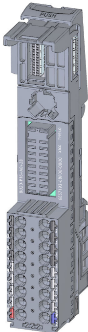
Figure 7-31 BU type U0, dark-colored version, without AUX terminals
