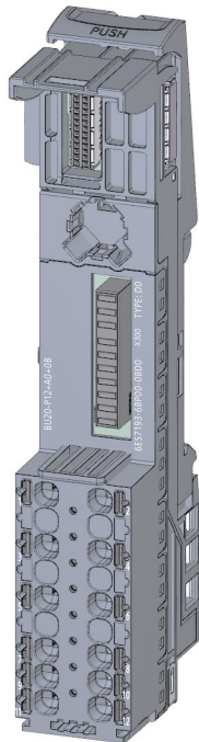
Figure 7-25 BU type D0, dark-colored version, without AUX terminals, supply over supply terminals
