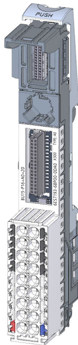
Figure 7-3 BU type A0, light-colored version, without AUX terminals
