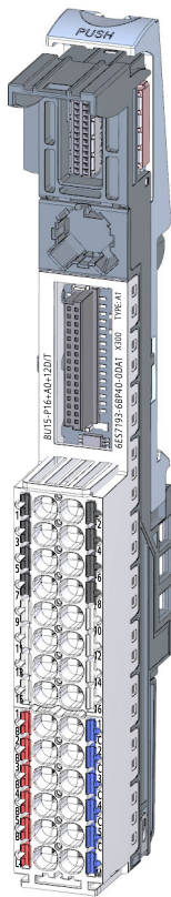
Figure 7-9 BU type A1, light-colored version, with add-on terminals
