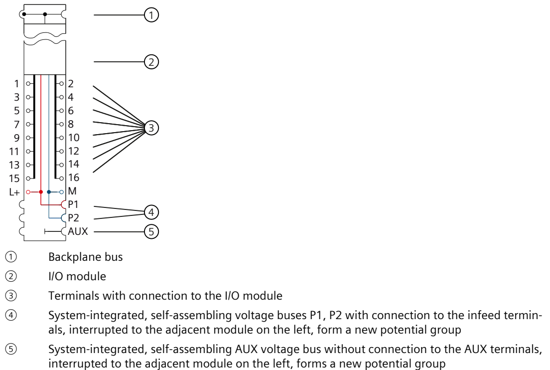
Figure 7-4 Block diagram of the BU type A0, light-colored version, without AUX terminals
