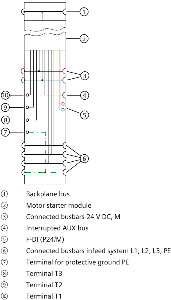
Figure 8-12 Block diagram of BaseUnit without infeed, with fail-safe input
