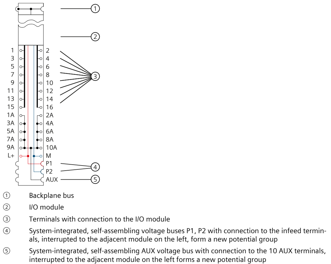
Figure 7-2 Block diagram of the BU type A0, light-colored version with AUX terminals
