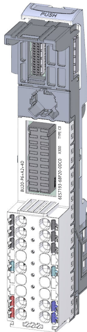
Figure 7-21 BU type C0, light-colored version, with AUX terminals, supply over supply terminals
