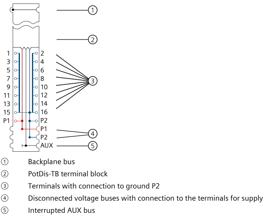
Figure 9-6 Block diagram of the PotDis-BU type P2, light-colored version
