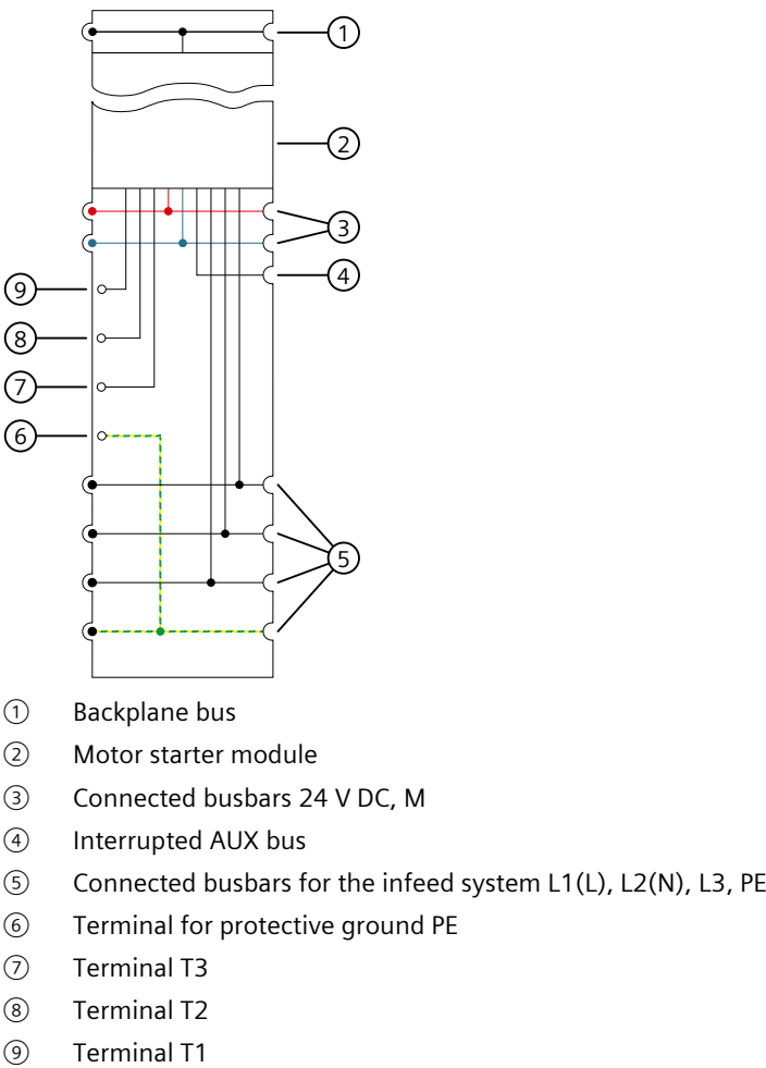
Figure 8-8 Block diagram BaseUnit without infeed
