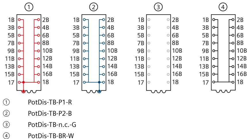
Figure 9-10 PotDis-TB block diagram
