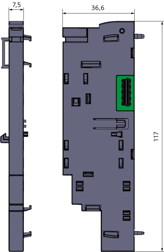
Figure B-4 Dimension drawing IO adapter
