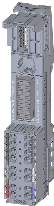
Figure 7-19 BU type B1, dark-colored version, without AUX terminals, supply over supply terminals
