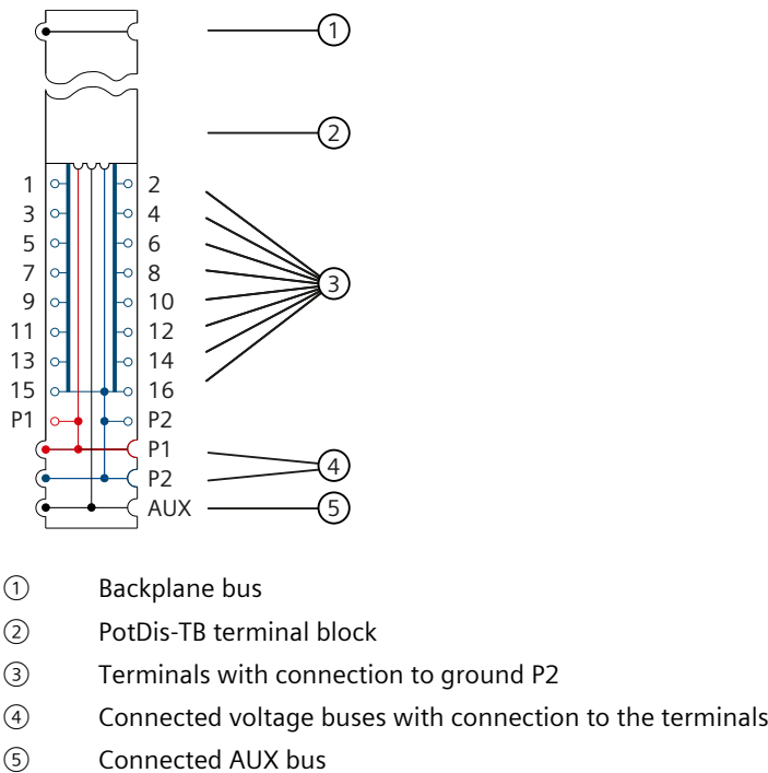
Figure 9-8 Block diagram of the PotDis-BU type P2, dark-colored version
