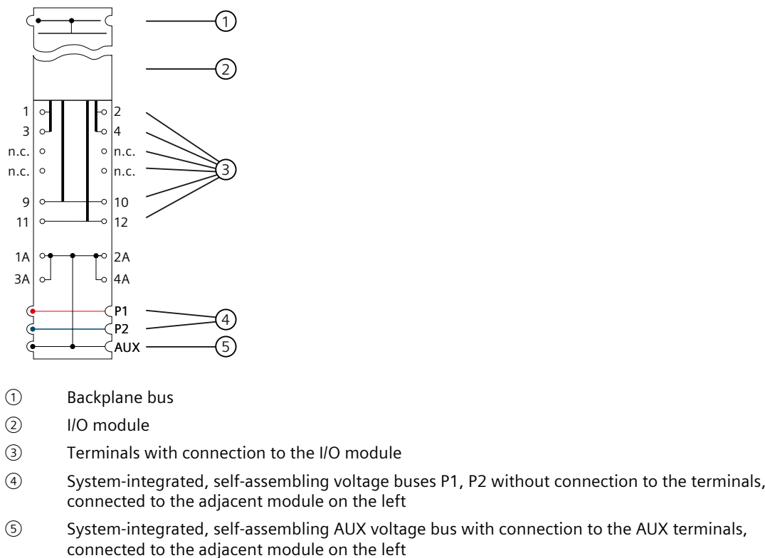
Figure 7-28 Block diagram of the BU type F0, dark-colored version, with AUX terminals, supply over supply terminals
