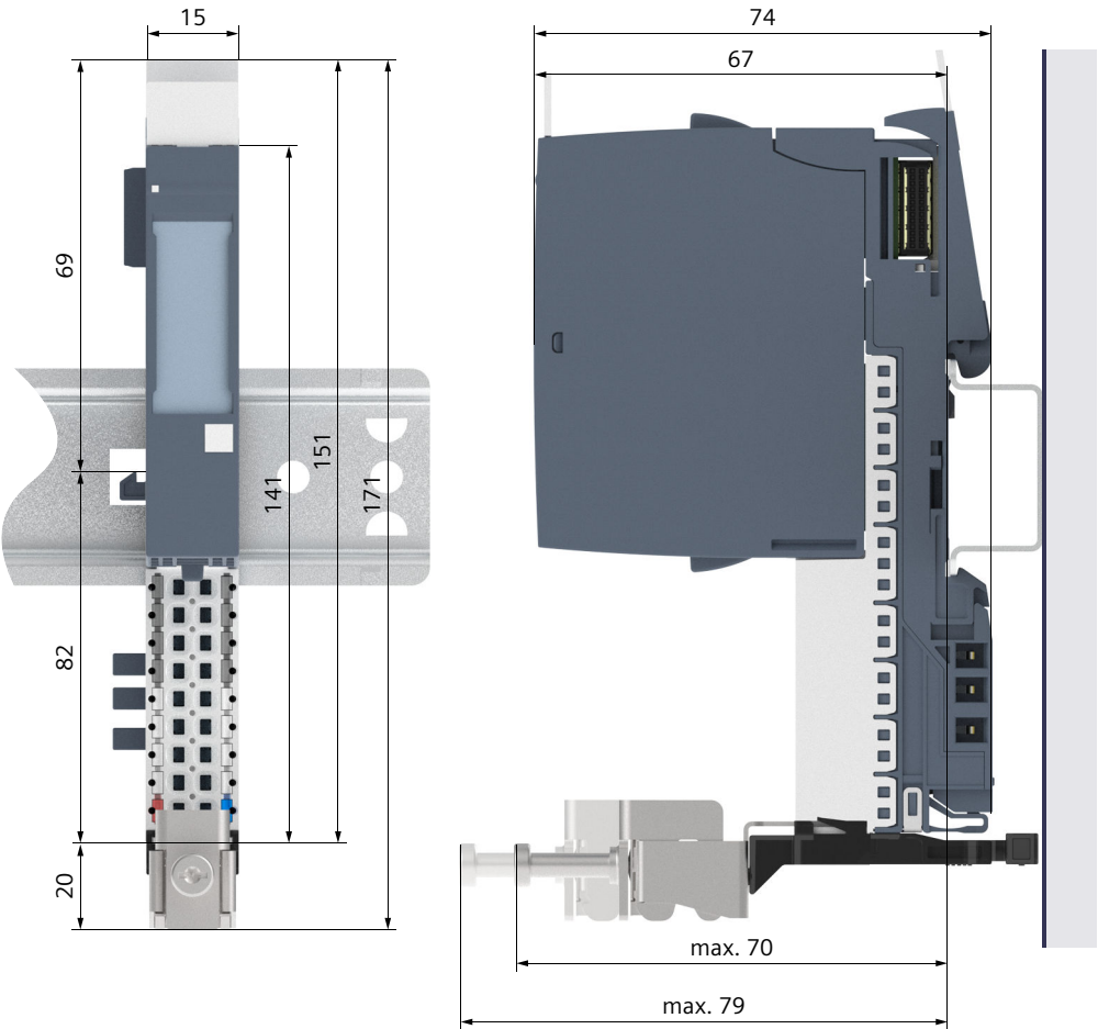
Figure C-2 Dimension drawing BU15-P16+A0+2D
