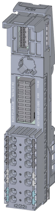
Figure 7-17 BU type B0, dark-colored version, with AUX terminals, supply over P1, P2 busbar
