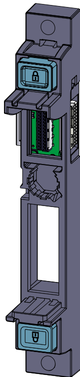
Figure 6-1 BaseCarrier type A0, light-colored version
