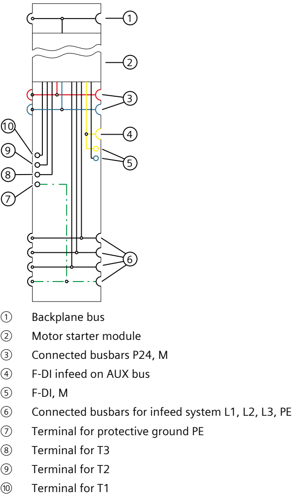
Figure 8-20 Block diagram of BaseUnit with F-DI infeed
