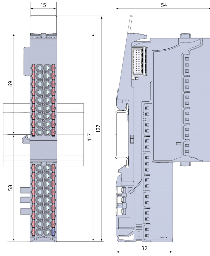
Figure E-1 Dimension drawing of PotDis BU-P1/B-R with plugged-in terminal block
