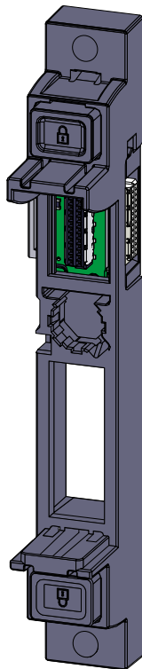
Figure 6-2 BaseCarrier type A0, dark-colored version
