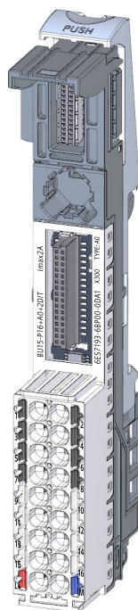
Figure 7-11 BU type A1, light-colored version, without add-on terminals
