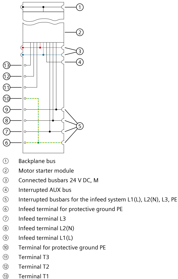
Figure 8-4 Block diagram of BaseUnit with 500 V AC infeed
