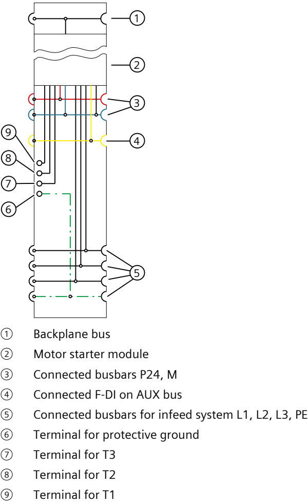
Figure 8-18 Block diagram of BaseUnit with F-DI routing
