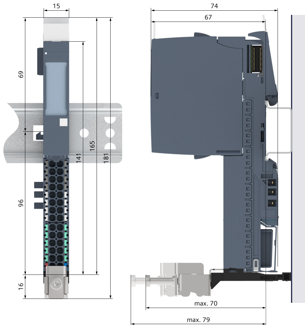
Figure C-1 Dimension drawing BU15-P16+A10+2D
